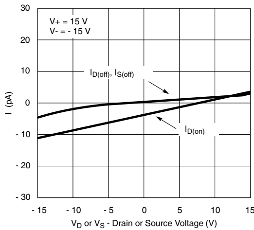
Leakage Current vs. Analog Voltage
