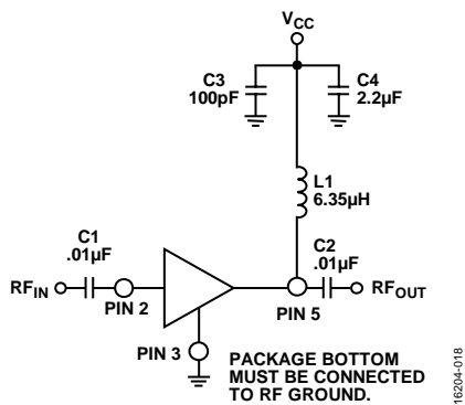
Figure 18. Evaluation Board Schematic
