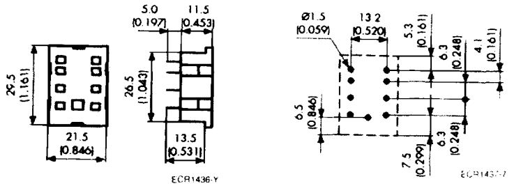
Mounting hole layout View from the wiring side
