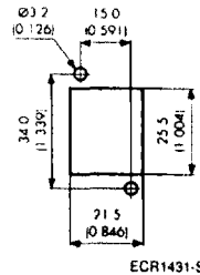
Mounting hole layout
