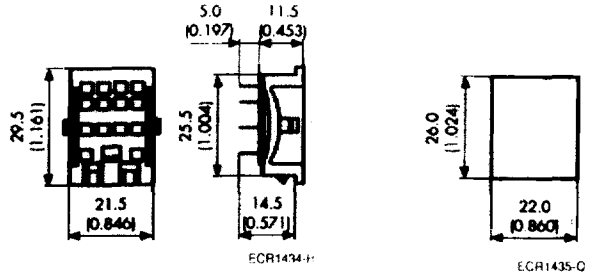
Mounting hole layout
