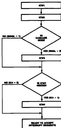
Figure 6. Initialization Sequence
