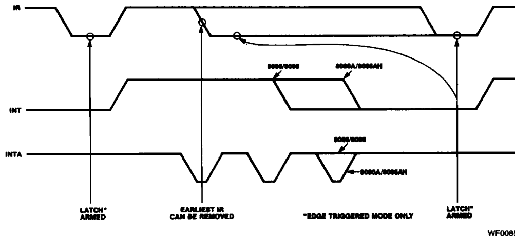
Figure 10. IR Triggering Timing Requirements
