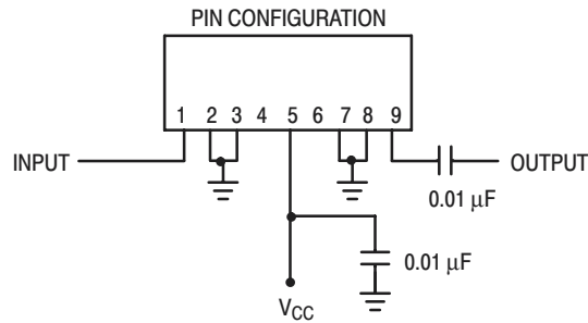
Figure 1. External Connections
