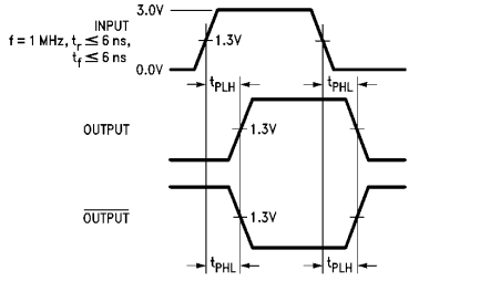
FIGURE 2. Propagation Delays
