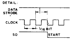
Fig.5 UAR/T TRANSMITTER TIMING
