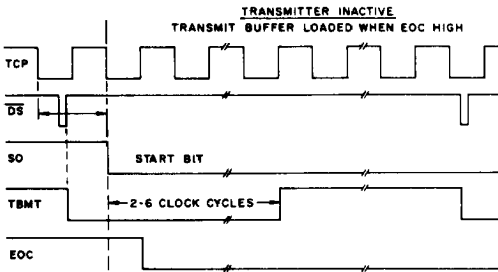
Fig.6 TRANSMITTER AT START BIT
