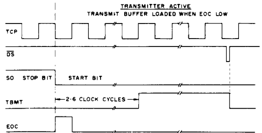
Fig.7 TRANSMITTER AT START BIT
