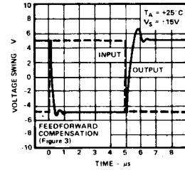
Inverter Pulse Response
