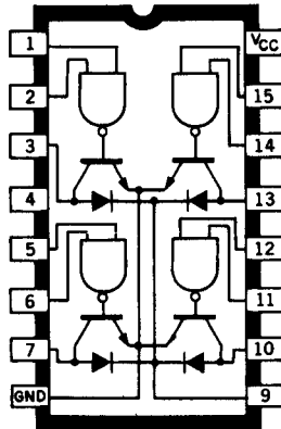
QUAD AND DRIVER
