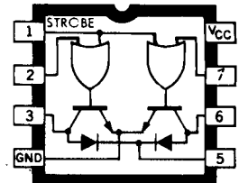
DUAL NOR DRIVER
