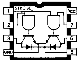
DUAL NAND DRIVER
