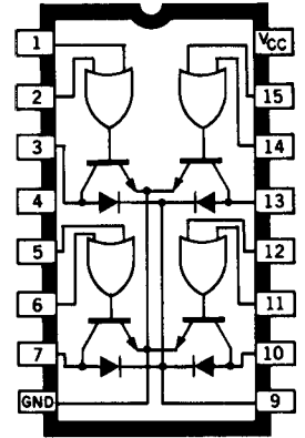
QUAD NOR DRIVER
