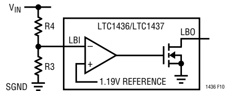
Figure 10. Low Battery Comparator
