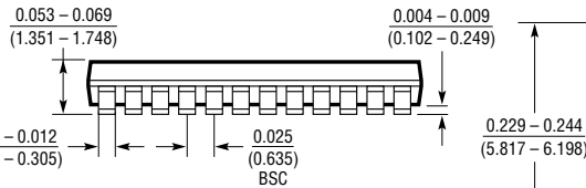
GN Package 24-Lead Plastic SSOP (Narrow 0.150) (LTC DWG # 05-08-1641)
