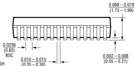
GW Package 28-Lead Plastic SSOP (Wide 0.300) (LTC DWG # 05-08-1642)
