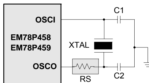
Fig. 19 Circuit for Crystal/Resonator
