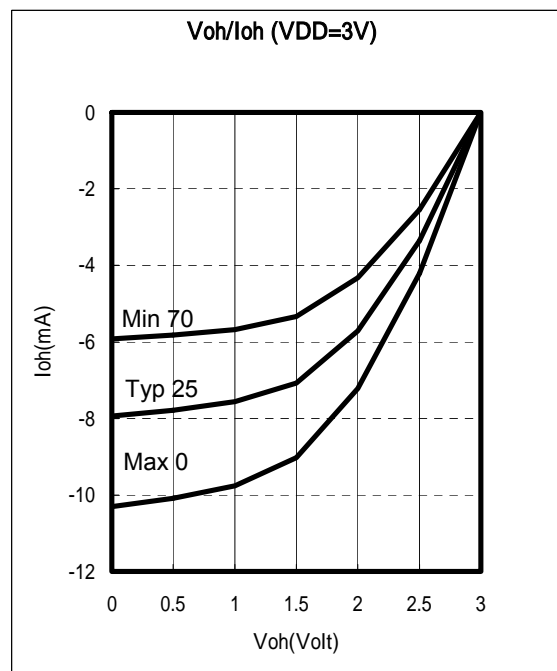
Fig.29 Port5, Port6, Voh vs. Ioh, VDD=3V
