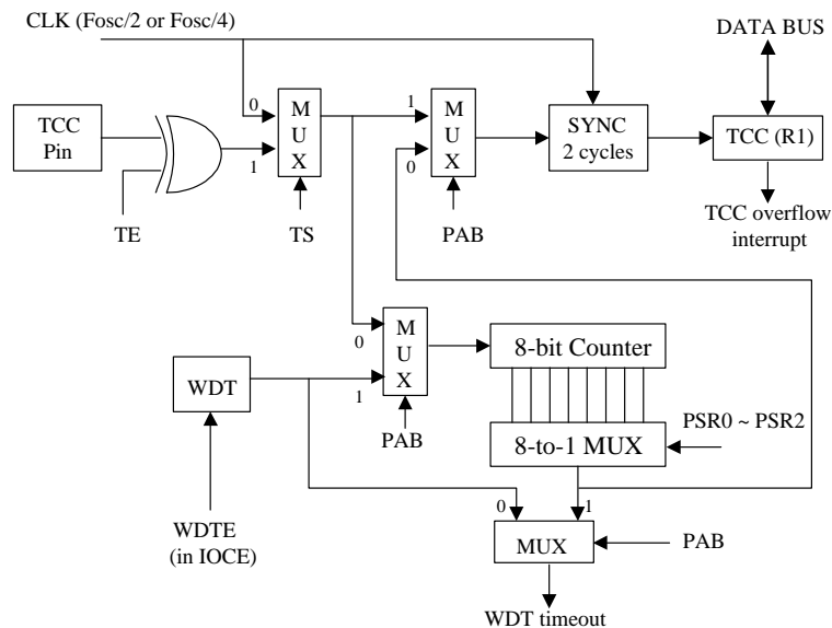
Fig. 5 Block Diagram of TCC and WDT
