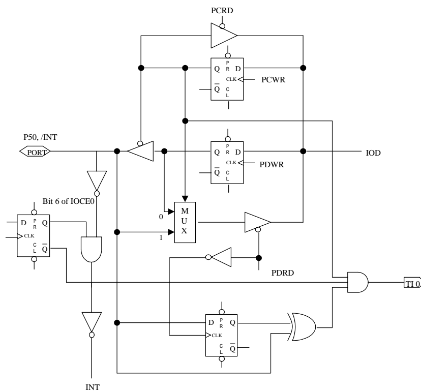
Fig. 7 The Circuit of I/O Port and I/O Control Register for P50(/INT)
