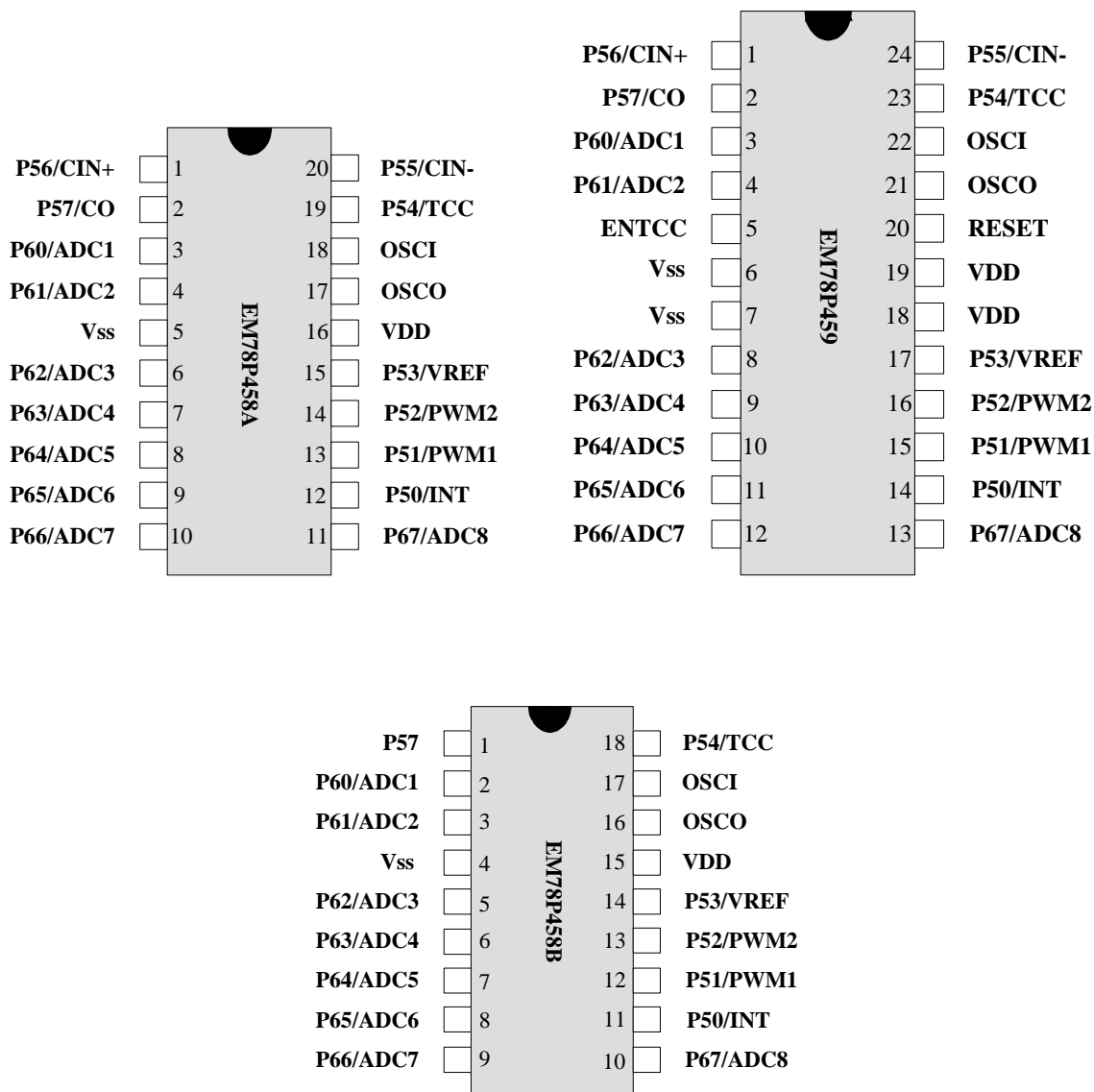
Fig. 1 Pin Assignment
