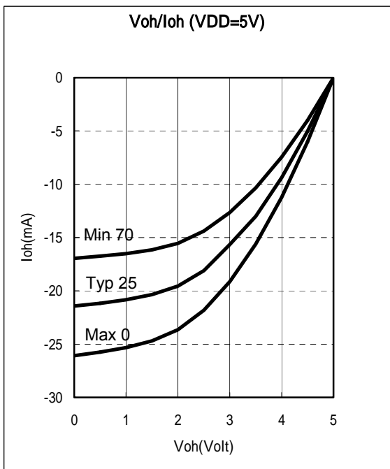
Fig.28 Port5, Port6, Voh vs. Ioh, VDD=5V
